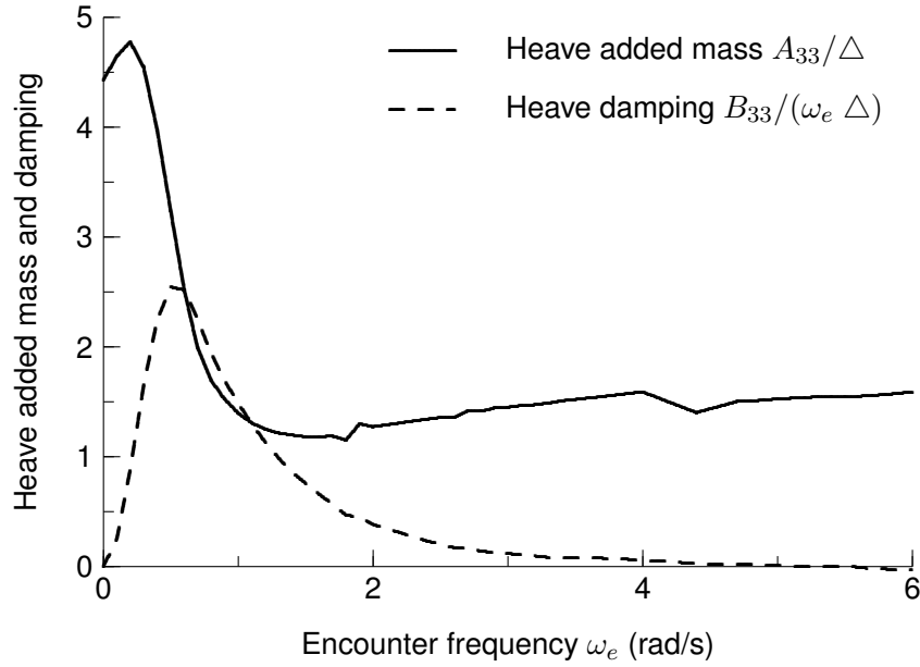
Figure 11: Heave Added Mass and Damping for Generic Frigate
